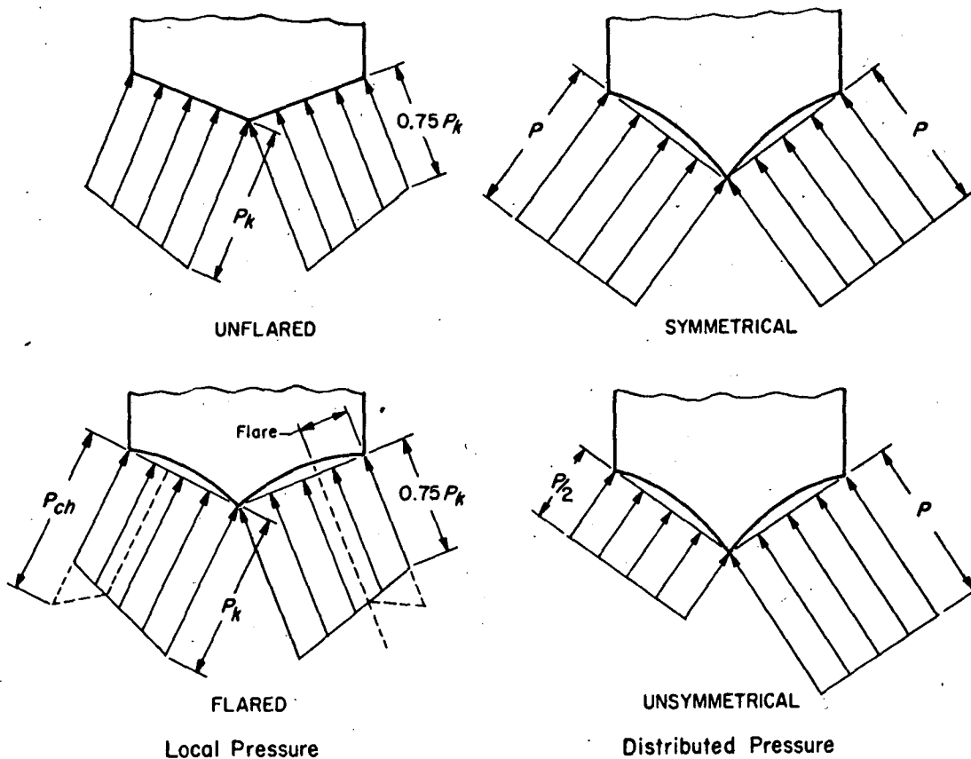
FIGURE 3. Transverse pressure distributions.
